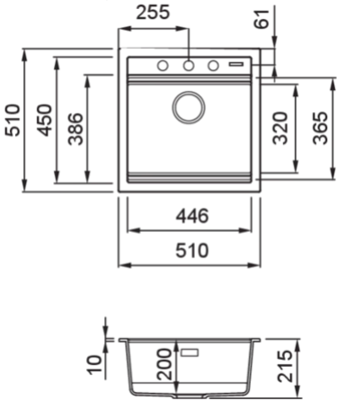
Technical Drawing
