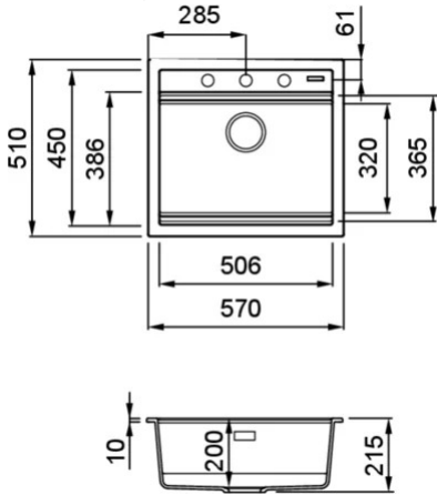
Technical Drawing
