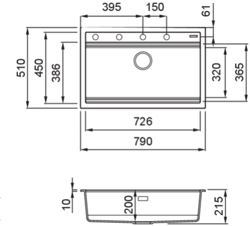
Technical Drawing
