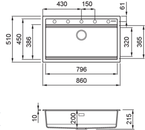
Technical Drawing
