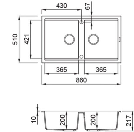
Technical Drawing
