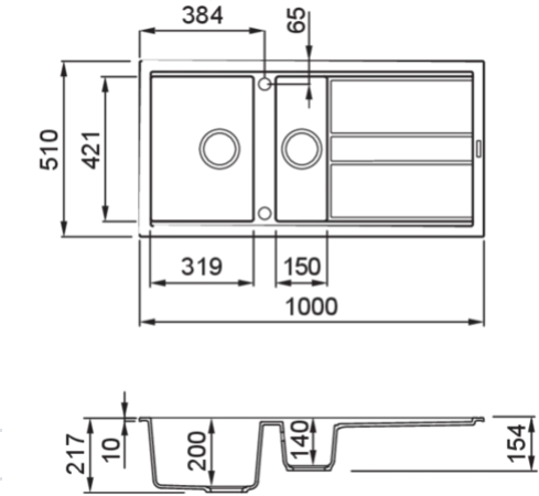
Technical Drawing
