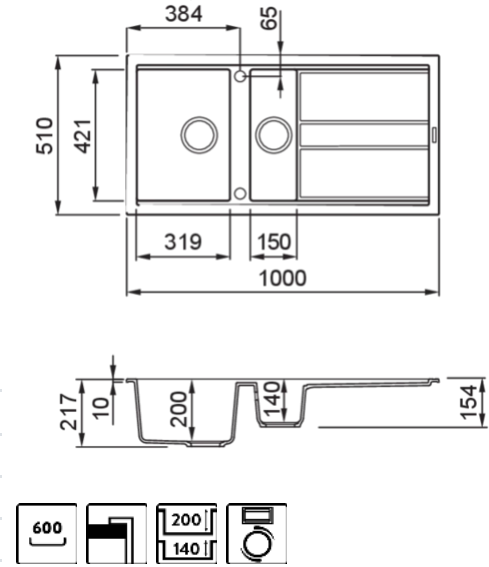
Technical Drawing
