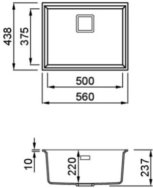
Technical Drawing
