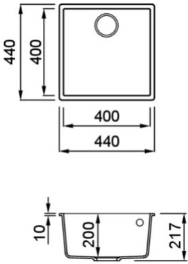
Technical Drawing
