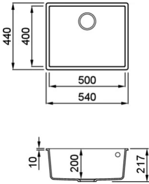
Technical Drawing
