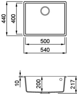
Technical Drawing
