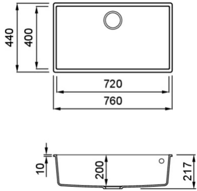
Technical Drawing
