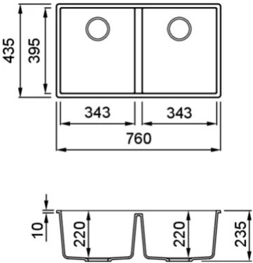
Technical Drawing
