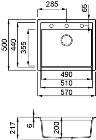
Technical Drawing
