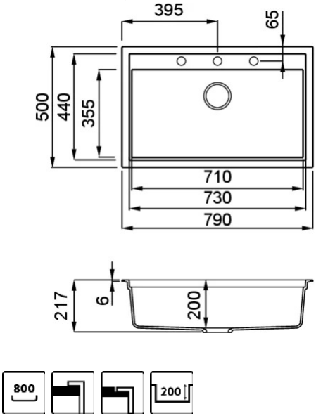
Technical Drawing
