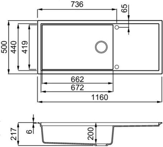
Technical Drawing
