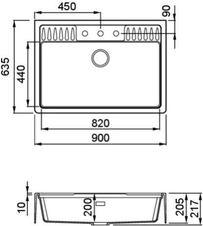
Technical Drawing
