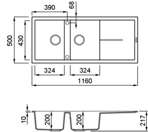
Technical Drawing
