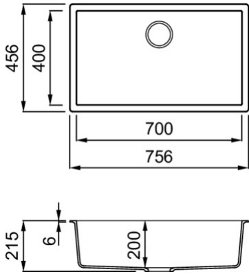
Technical Drawing
