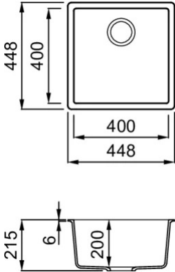
Technical Drawing
