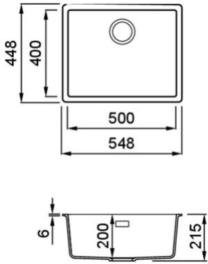
Technical Drawing
