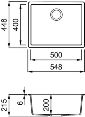
Technical Drawing
