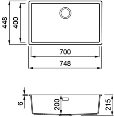
Technical Drawing
