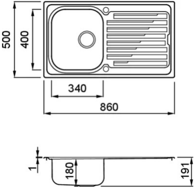
Technical Drawing
