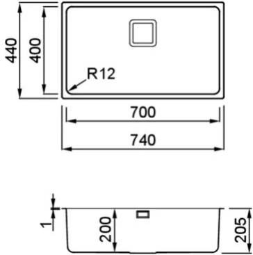
Technical Drawing
